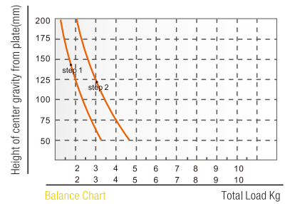
COUNTERBALANCE GRAPH
